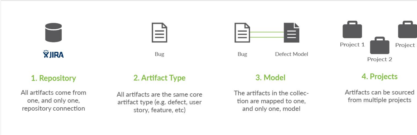
Figure 2: Collection Definition
